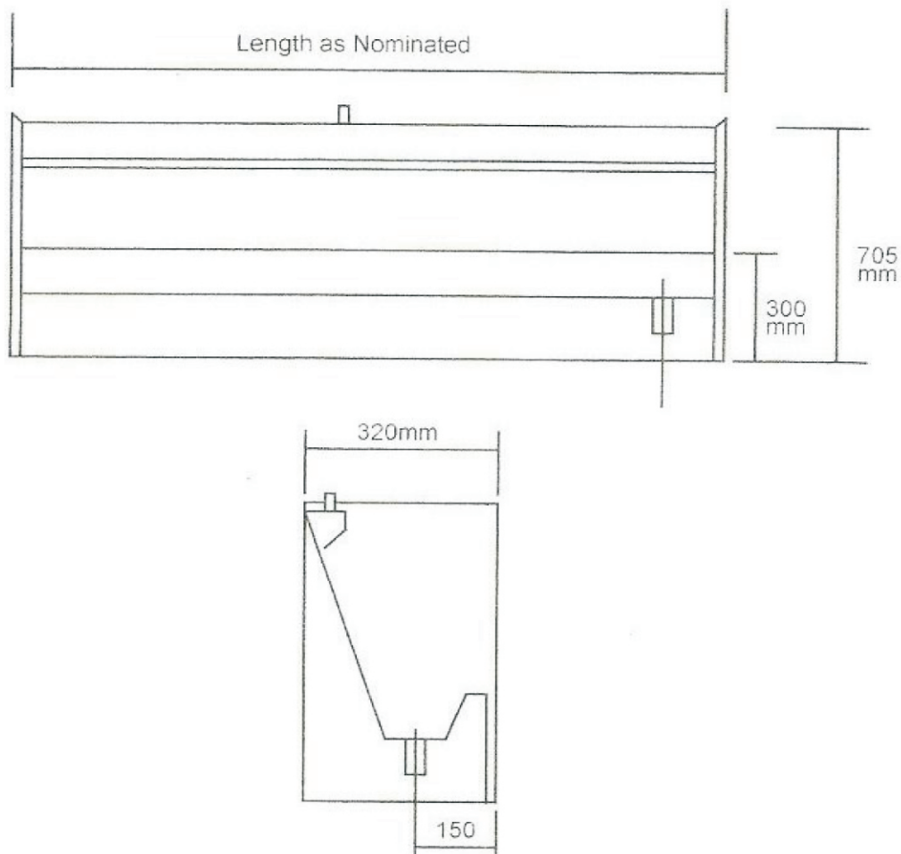
Wall Hung Slab Urinal.
