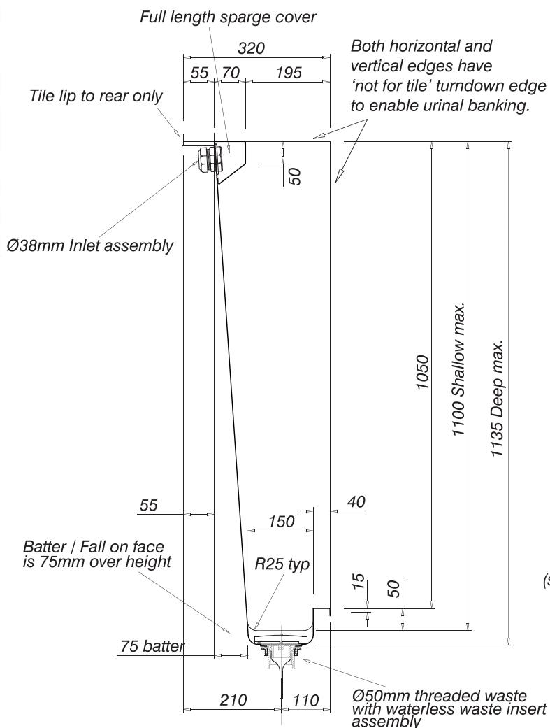
SECTION; WATERSAVING URINAL WASTE POSITION; STANDARD (Rear entry shown)
